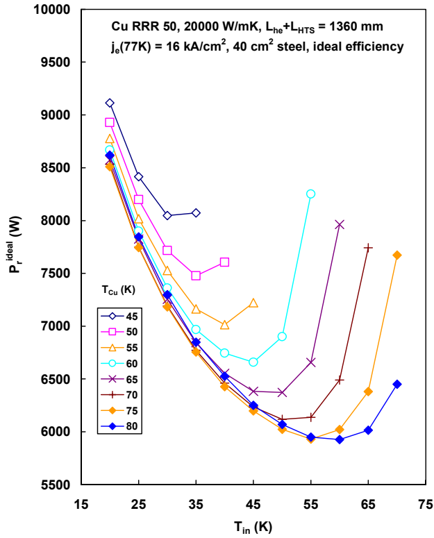
Fig. 16. Required refrigerator input power to cool the whole binary current lead versus the helium inlet temperature for copper temperatures in the 45 – 80 K range at the cold end. The data are for ideal cooling cycles.
