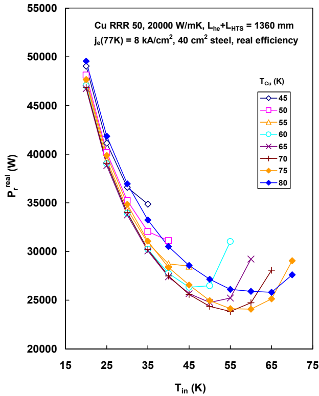
Fig. 23. Required refrigerator input power to cool the whole binary current lead versus the helium inlet temperature for copper temperatures in the 45 – 80 K range at the cold end. The data are for real cooling cycles.
