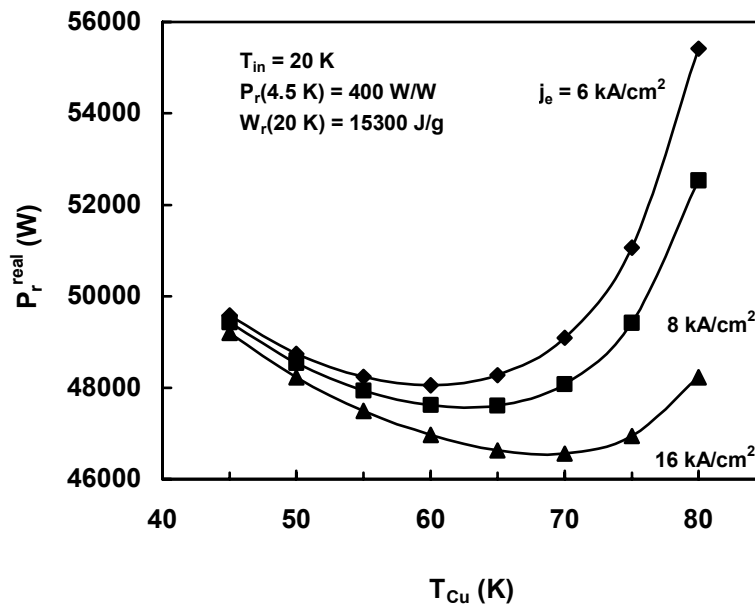
Fig. 33. Refrigerator input power required to cool current leads constructed of AgAu/Bi-2223 tapes with j_e(77 K, 0) values of 6, 8 and 16 kA/cm 2 . Due to the enhanced heat load caused by a larger superconductor cross-section the required refrigerator input power increases with decreasing j_e . The optimum conductor temperature at the cold end of the heat exchanger is shifted to lower values for reduced critical current densities.
