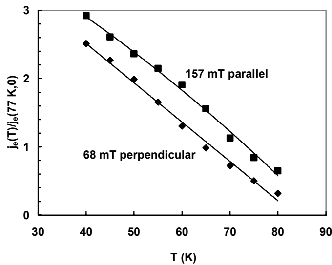
Fig. 4. Estimated engineering critical current densities of the AgAu/Bi-2223 tapes for magnetic fields of 157 mT parallel and 68 mT perpendicular to the tape surface normalised to the j_e value at 77 K and B = 0 . The current carrying capacity of the current lead is limited by the magnetic field perpendicular to the tape surface.
