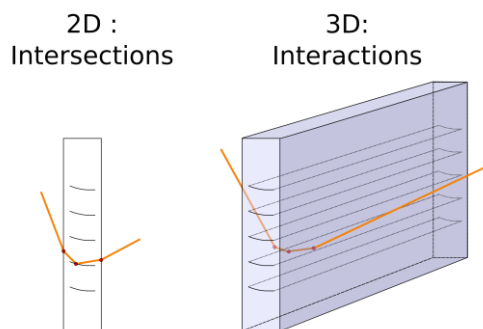
Figure 2: Illustration of the mixed dimensionality concept for ray tracing of profile defined geometries.
