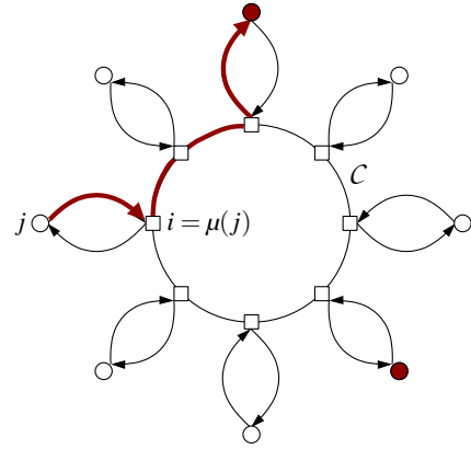
Figure 1: Core connection game instance. Marked client nodes are drawn in bold. The flow of j in the routing scheme is indicated by the bold path.
