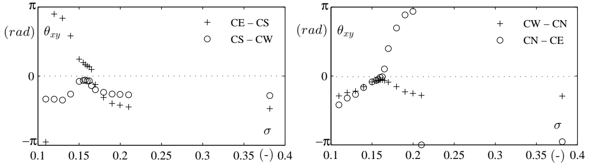
Figure 5: Phase shift at the precession frequency for 4 pairs of pressure signals measured in the draft tube cone as a function of the cavitation number ( Fr = 8.75 ).
