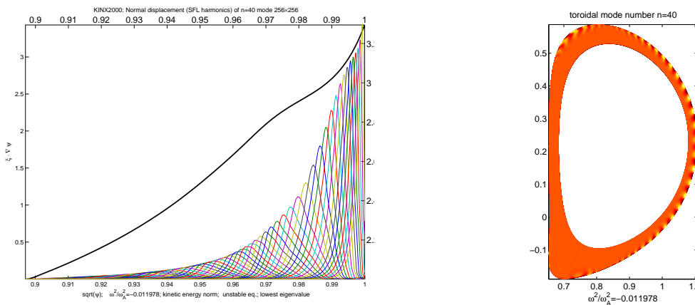
Fig.2.4 The kink/ballooning mode structure for the TCV shot #26383. Normal displacement harmonics in straight magnetic field line coordinate (a) and level lines of the normal displacement.
