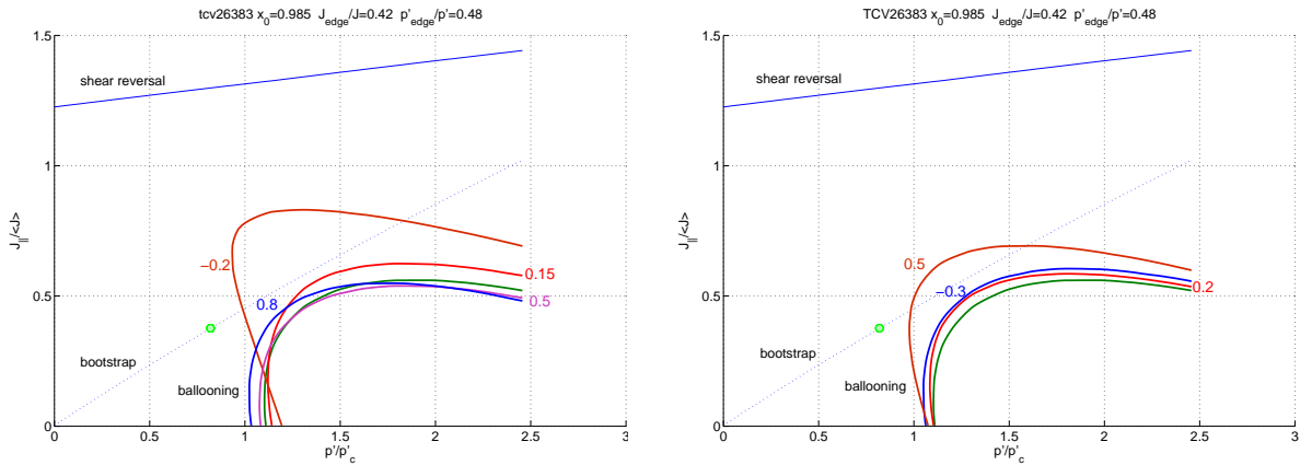
Fig.2.3 The n = \infty stability limit in the parametric plane. The local limit at \sqrt{\psi} = 0.985 is shown. Triangularity (a) and squareness (b) variations. Different curves correspond to different values of triangularity and squareness respectively.
