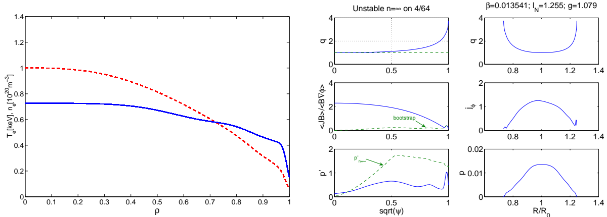
Fig.1.1 The electron temperature and density profiles for the TCV shot #26383 (a). Plasma profiles for the reference equilibrium (b).
