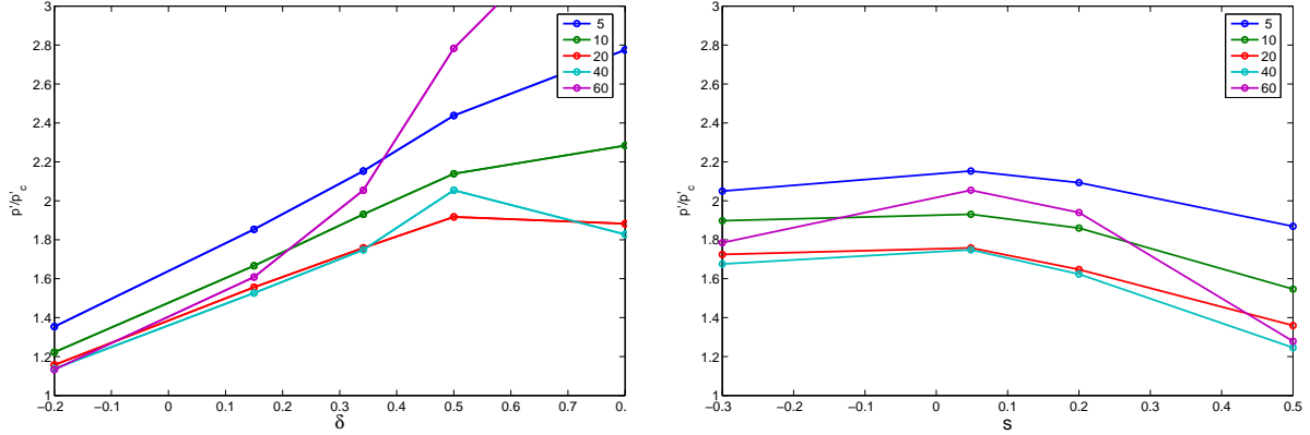
Fig.2.2 The stability limit in p'/p'_c at the bootstrap line under triangularity (a) and squareness (b) variations. Different curves correspond to different toroidal wave numbers.
