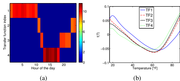
Fig. 8. Results on the GEFCom data with L = 4 . (a) \Lambda_{\text{temp}} matrix showing the activation of the temperature transfer functions for the 24 hours per day. (b) Shapes of the estimated week temperature transfer functions.
