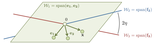
Fig. 2. Example where a set of non-zero measure is wrongly classified, when the \ell_1 norm is used in the sparse coding step.
