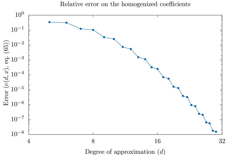
Figure 2: Relative error of the homogenized coefficients, e(d, x) , see Eq. (65), for the fast/slow SDE (63) at x = (0.2, 0.2) . In this case, the convergence is also super-algebraic.
