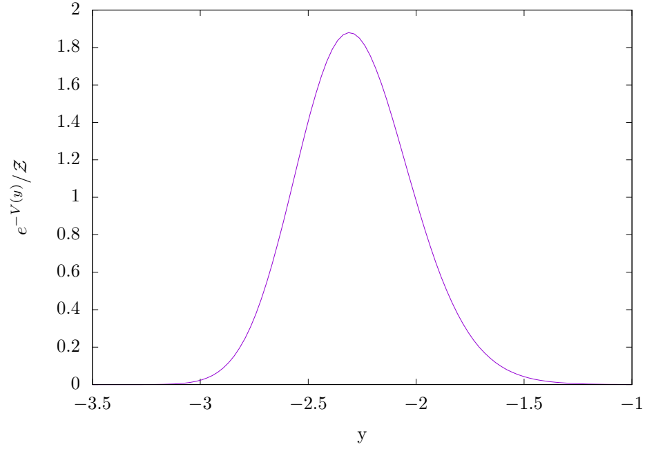
Figure 4: Probability density e^{-V(\cdot)}/\mathcal{Z} associated to the potential (68).
