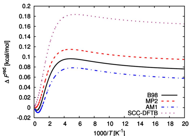
FIG. 6. Reduced reaction free energies of the first step of [1,5] hydrogen shift reaction in (3Z)-(5,5,5- H_3 )penta-1,3-diene ( 1-5,5,5- d 3 ) calculated in the HA as the Boltzmann average of all s-trans and s-cis isomers.
