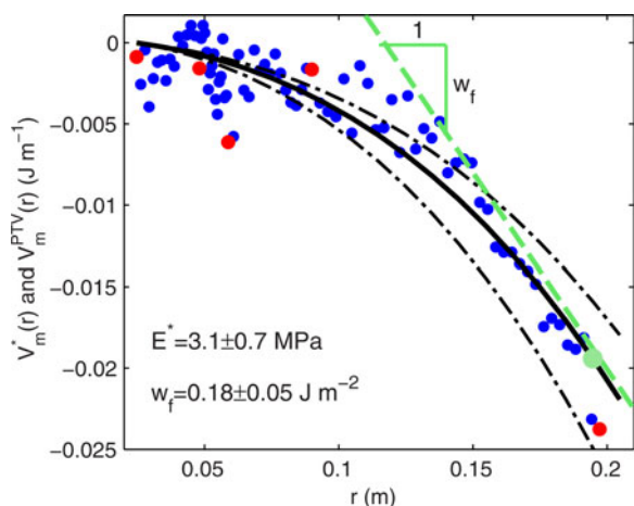
Fig. 7. Derived mechanical energy with crack length r for the experiment shown in Figure 5. The red dots represent the key frames at which the saw cut length r was estimated from the images. The black line represents the best fit of V_m^*(r) (Eqn (7)) to the experimental data V_m^{PTV}(r) (Eqn (6), blue dots), and the black dashed-dotted lines the 95% confidence interval. The green dashed line represents the tangent to the mechanical energy at r = r_c = 0.2 m.
