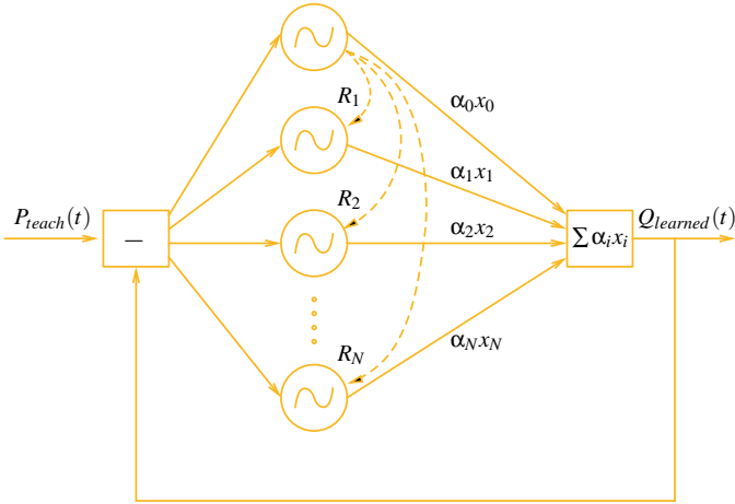
Fig. 3. This figure shows the structure of the network of adaptive Hopf oscillators after we added coupling. Each oscillator receives the same learning signal F(t) = P_{teach}(t) - \sum_i \alpha_i x_i , which is the difference between the signal to be learned, P_{teach}(t) , and the signal already learned, Q_{learned}(t) . Then all the oscillators (except oscillator 0) receive the scaled phase input R_i from oscillator 0. Refer to Equations (13)-(18) and to the text for more details.
