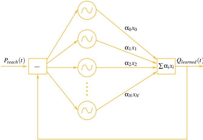
Fig. 2. This figure shows the structure of the network of adaptive Hopf oscillators. Each oscillator receives the same learning signal F(t) = P_{teach}(t) - \sum_i \alpha_i x_i , which is the difference between the signal to be learned, P_{teach}(t) , and the signal already learned, Q_{learned}(t) . Refer to Equations (4)-(8) and to the text for more details.
