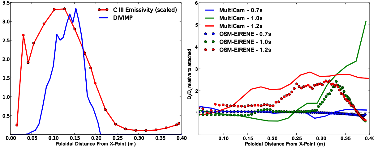
Figure 6: (left) comparison of measured C III line emissivity along the outer divertor leg measured at 1.0s with the result from a DIVIMP simulation (right) comparison of measured D_\gamma/D_\alpha line emissivity ratio profiles with output from OSM-EIRENE simulations.
