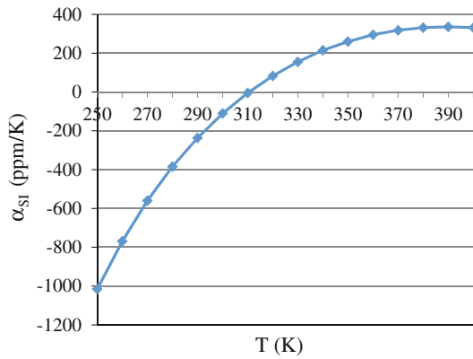
Fig. 7 Temperature coefficient \alpha_{S_I} (ppm/K) of S_I versus temperature
