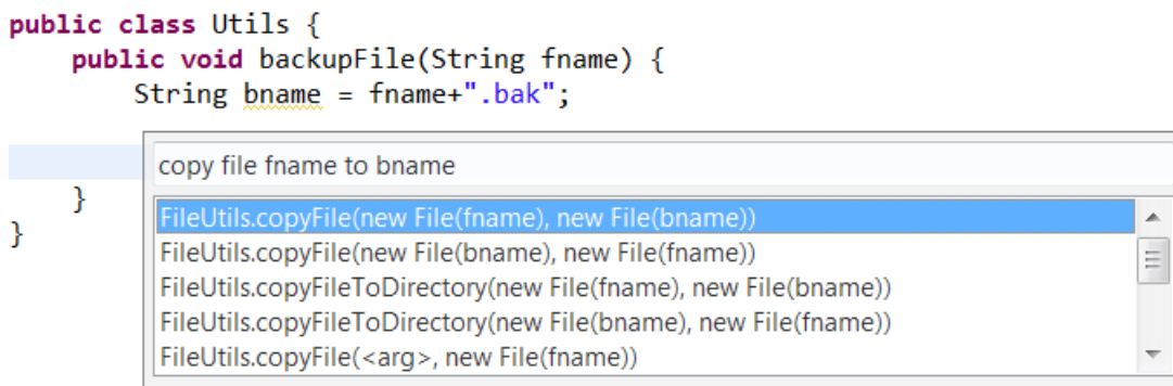
Figure 3.1: After the user inserts text input, anyCode suggests five highest-ranked well-typed expressions that it synthesized for this input.
